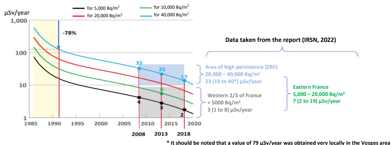
Figure 12: Trend in the average external dose ( \mu\text{Sv}/\text{year} ) estimated here for an adult working outdoors in a rural environment according to the surface activity of deposited Cs-137 ( \text{Bq}/\text{m}^2 ) and comparison with dose estimates from the report (IRSN, 2022) for the period 2008-2018
