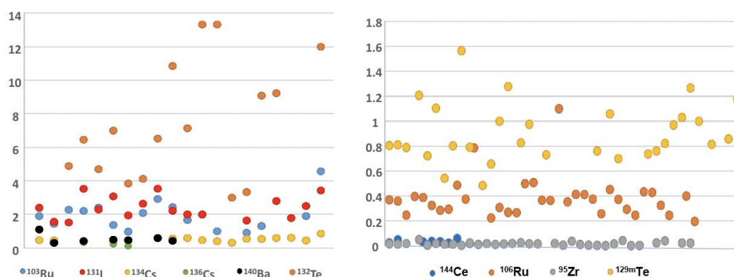
Figure 5: Activity concentrations in air of 10 radionuclides compared with those of 137 -Cs
