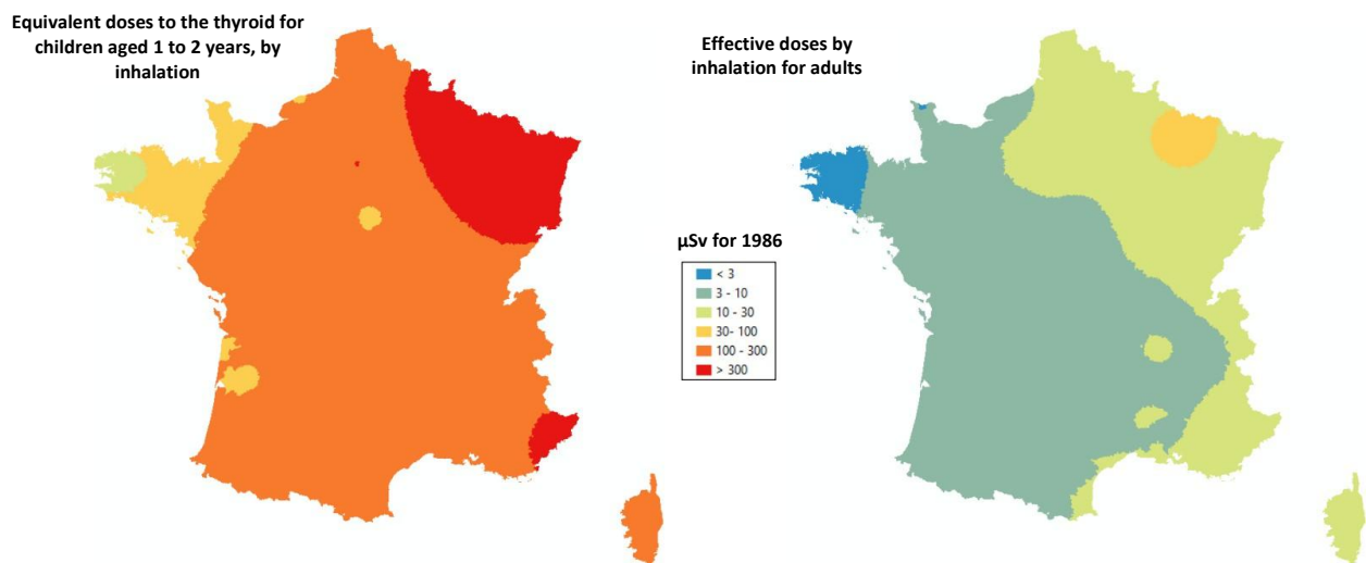
Figure 7: Average effective doses received by inhalation in 1986 for adults (right-hand map) and equivalent doses to the thyroid for children (left-hand map) aged 1 to 2 years ( \mu\text{Sv} ).
