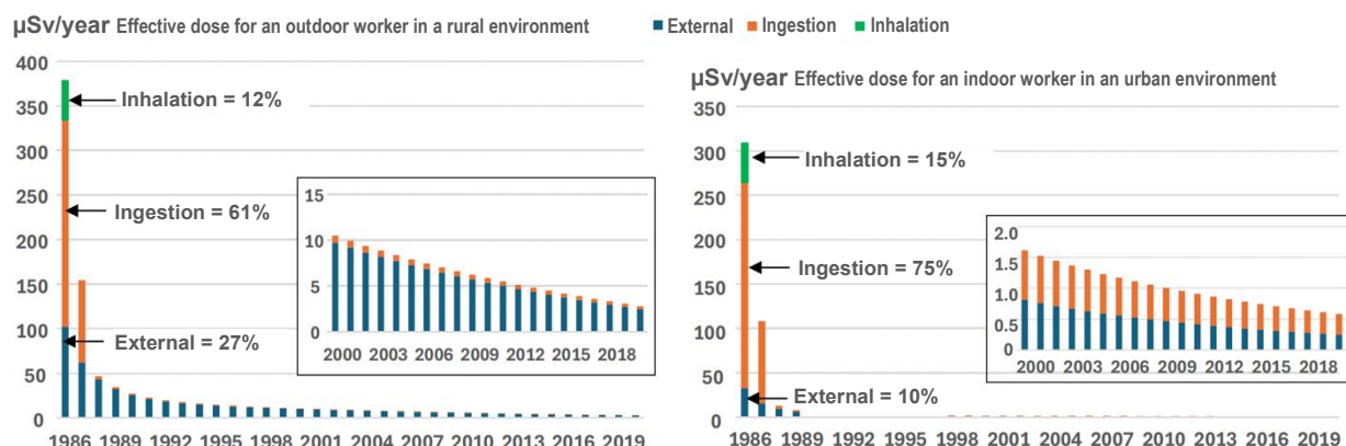
Figure 26: Trend in average total effective dose, all exposure pathways combined, estimated for adults, one working outdoors in a rural environment (left graph), the other working indoors in an urban environment (right graph), in the vicinity of Verdun
