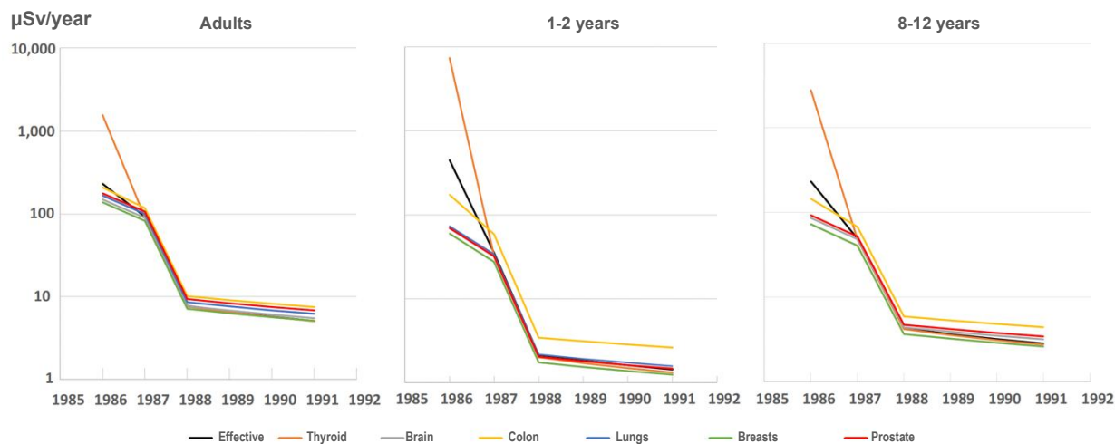
Figure 25: Comparison of trends in average equivalent doses to the various organs received by ingestion and estimated for adults, children aged 1 to 2, and children aged 8 to 12 ( \mu\text{Sv/year} )
