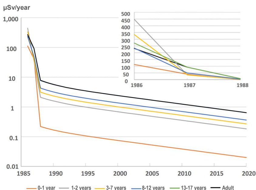
Figure 23: Comparison of trends in average effective doses estimated to be received by ingestion for various age groups ( \mu\text{Sv}/\text{year} )
