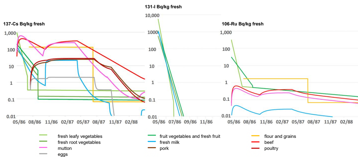
Figure 19: Examples of reconstruction by the SYMBIOSE model of the temporal trend of specific activities for radionuclides and foodstuffs for which few measurement results are available.
