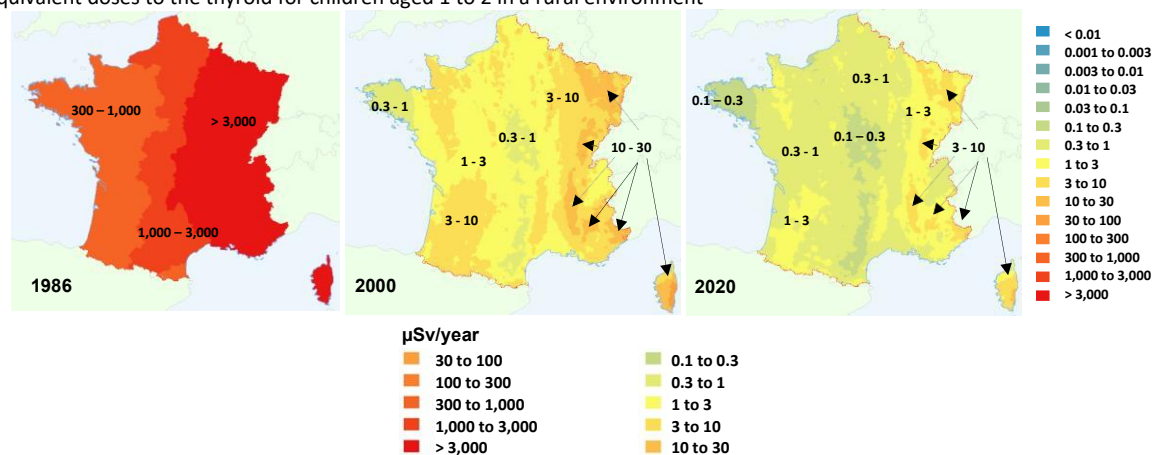
Figure 28: Average equivalent doses to the thyroid estimated for children aged 1 to 2 living in a rural environment in 1986, 2000 and 2020 (in µSv/year)
