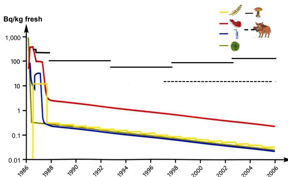
Figure 28: Overall trends in caesium-137 specific activities and activity concentrations in certain types of French foodstuffs (Bq/kg fresh; Renaud et al., 2007)
