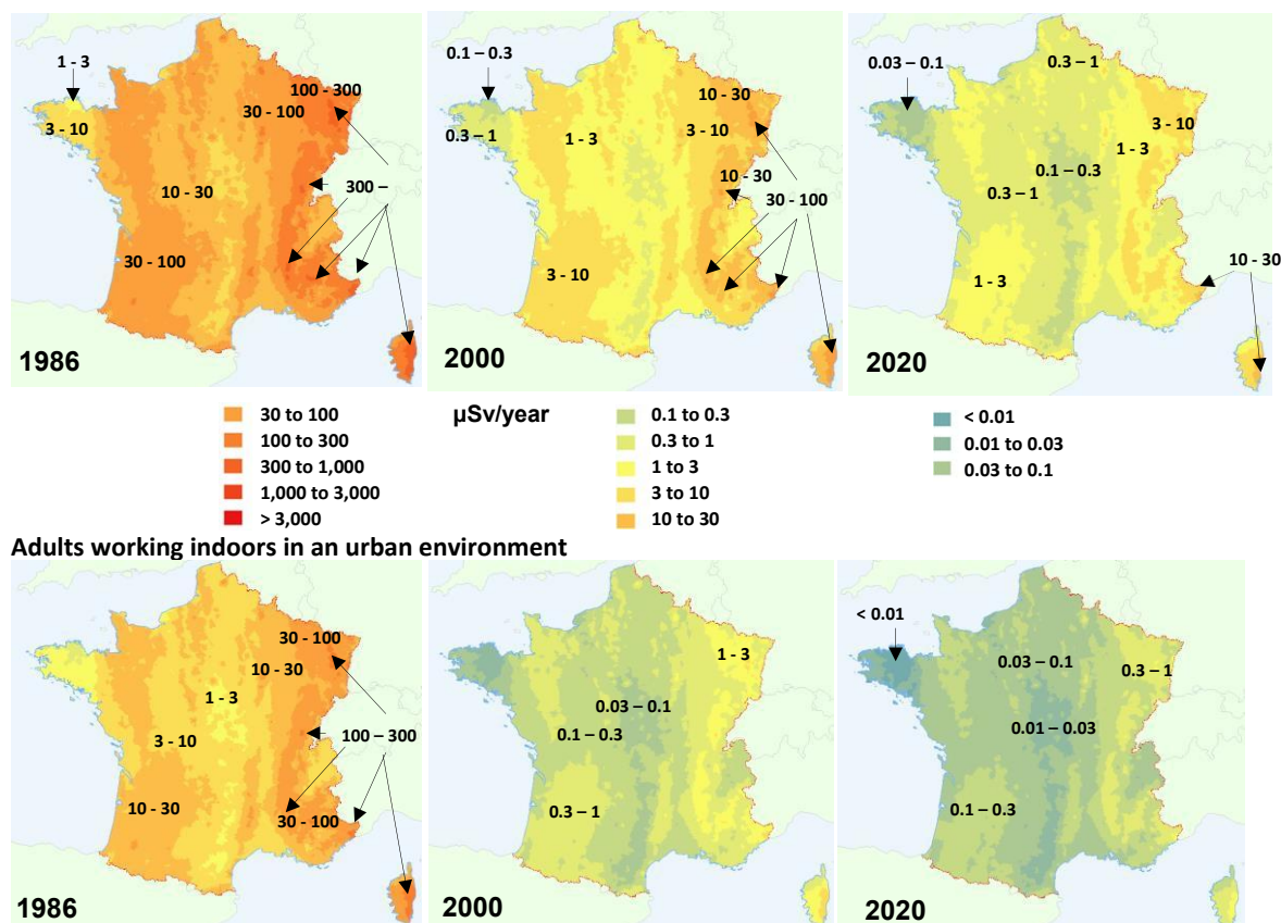
Figure 15: Mapping of average doses (μSv/year) due to external exposure for adults working outdoors in a rural environment or indoors in an urban environment for the years 1986, 2000 and 2020.
