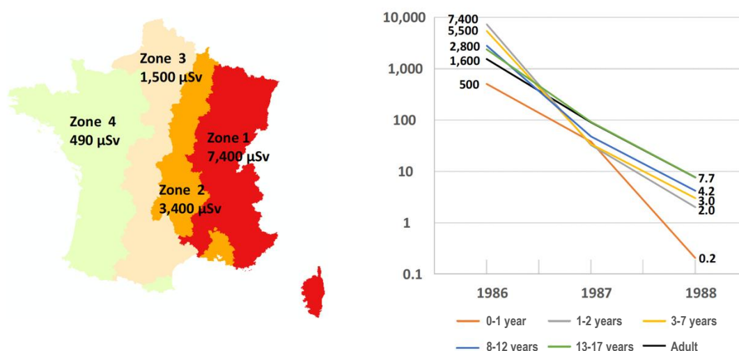
Figure 24: Map of average equivalent doses to the thyroid by ingestion (μSv/year) for children aged 1 to 2 in 1986, and comparison of trends between 1986 and 1988 for the various age groups
