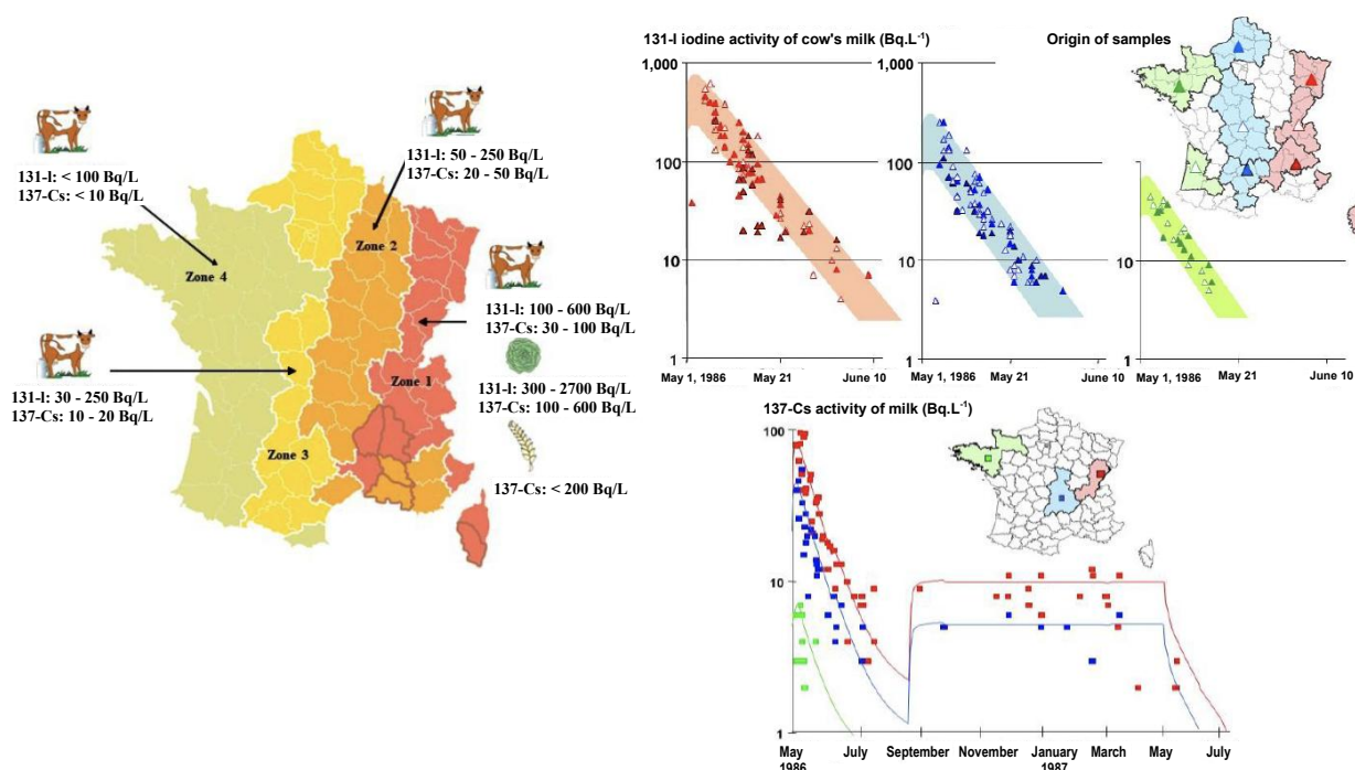
Figure 17: Zones of homogeneous specific activity and activity concentrations of iodine-131 and caesium-137 observed in 1986 in foodstuffs.
