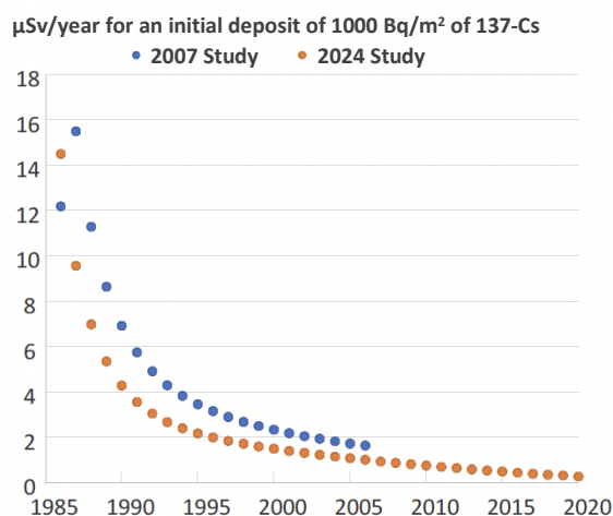
Figure 13: Comparison of changes in average external doses between the 2007 study and this update, all radionuclides combined, and for an initial deposit of 137-Cs of 1000 Bq/m 2 , estimated for an adult working outdoors in a rural environment.
