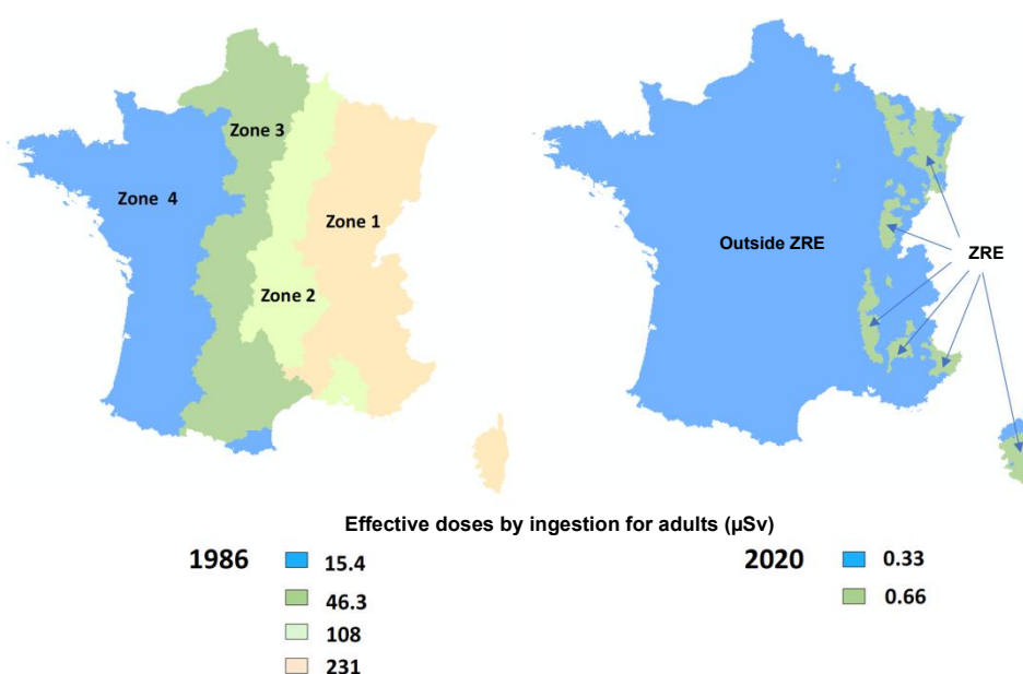
Figure 22: Average doses ( \mu\text{Sv}/\text{year} ) from ingestion of ^{137}\text{Cs}^+ , estimated for adults in 1986 and 2020
