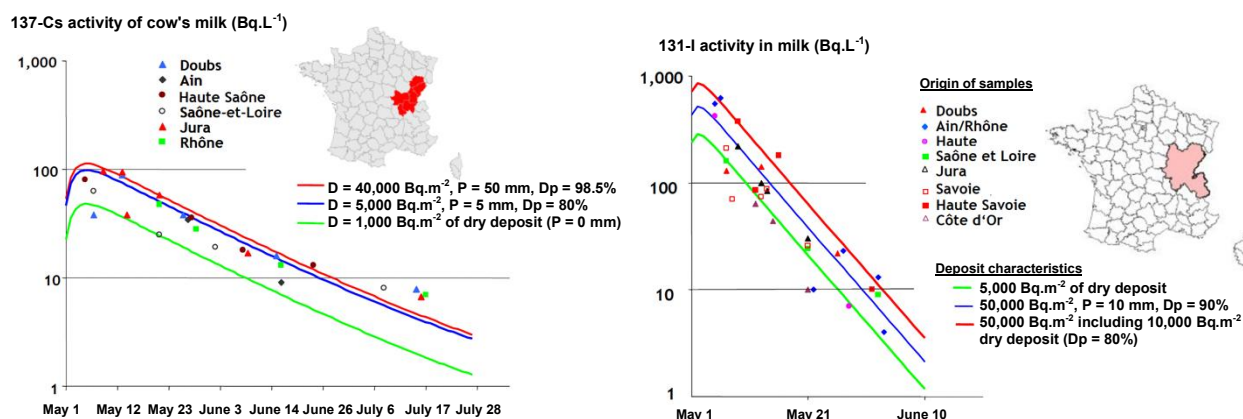
Figure 18: Examples of adjustment of simulations from the SYMBIOSE model (curves) to the 131 I and 137 Cs+ activities measured in 1986 in milk (points) according to the initial deposit and the département of origin of the samples
