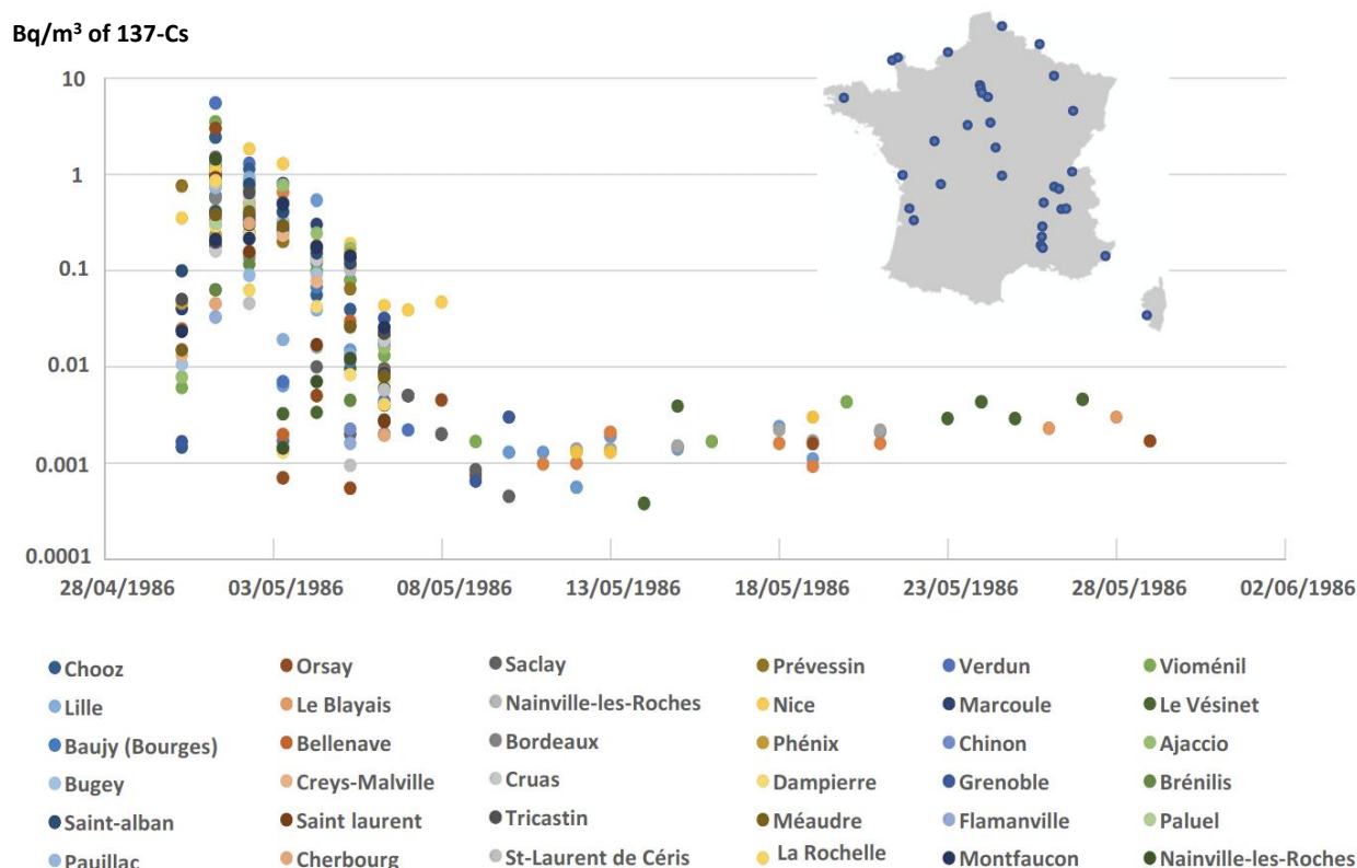
Figure 1: Activity concentrations of ^{137}\text{Cs} in the air measured on the daily filters of 36 aerosol sampling stations throughout France ( \text{Bq/m}^3 ).
