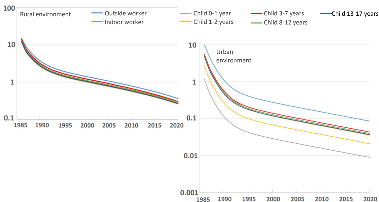
Figure 16: Trends in annual external doses as a function of time since the Chernobyl accident and by age group ( \mu\text{Sv/year} ), all radionuclides combined, and for an initial unit deposit of 1 \text{ kBq/m}^2 of caesium-137
