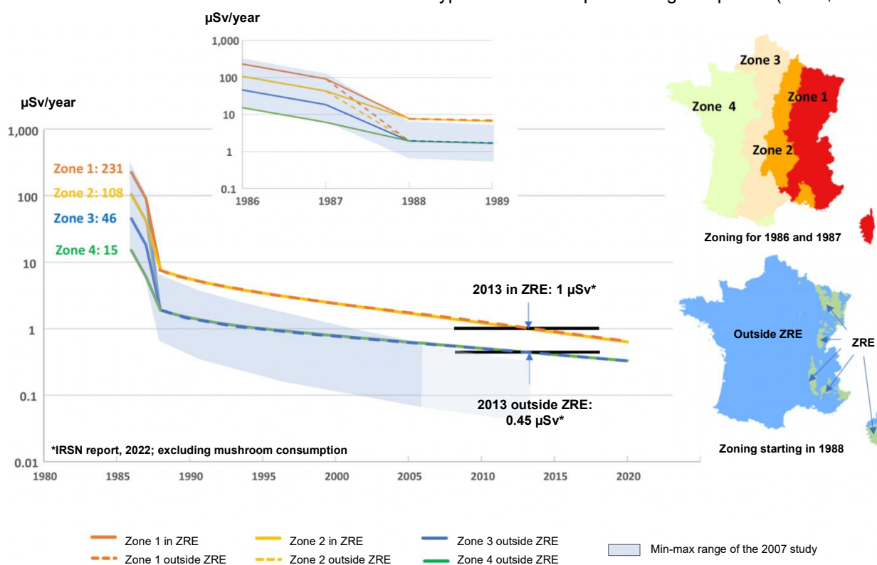
Figure 21: Trends in estimates of average doses received by ingestion of foodstuffs between 1986 and 2020 in \mu\text{Sv/year} and corresponding zones. ZRE: Area of high persistence.
