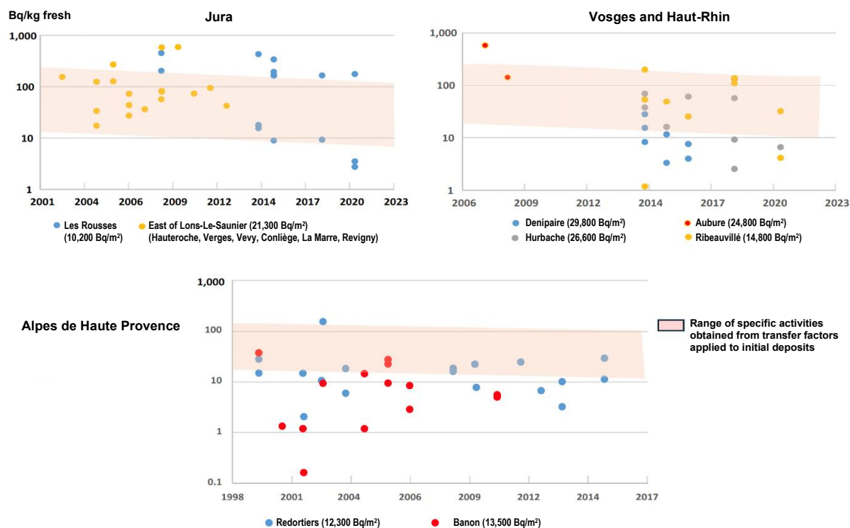
Figure 31: Caesium-137 specific activities (Bq/kg fresh) measured by ASNR (and its predecessors IPSN, OPRI and IRSN) in mushrooms collected in a number of municipalities or groups of municipalities in eastern France.
