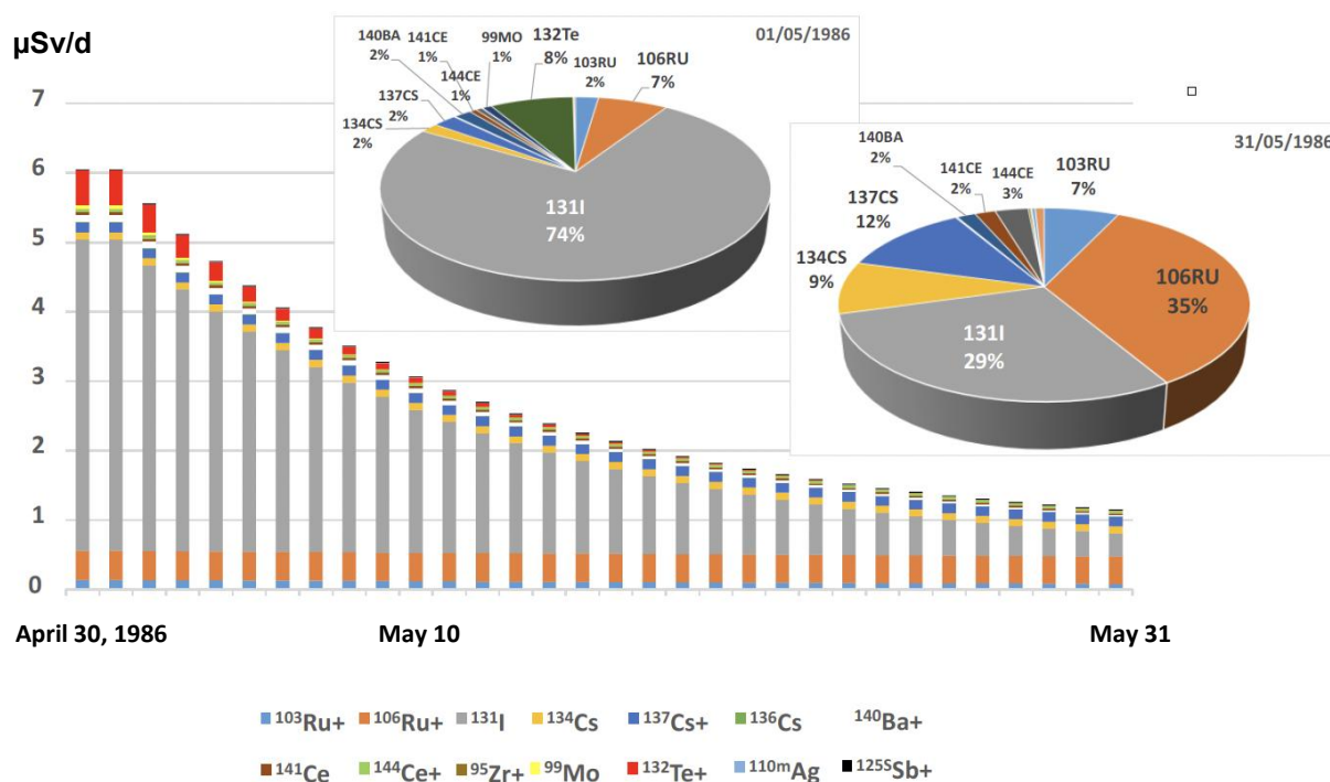
Figure 6: Trend in daily average effective doses received by inhalation by an adult during the month of May 1986 for a unit activity concentration of 1 Bq/m 3 of 137 -Cs and contribution of the various radionuclides measured in the air (µSv/d)
