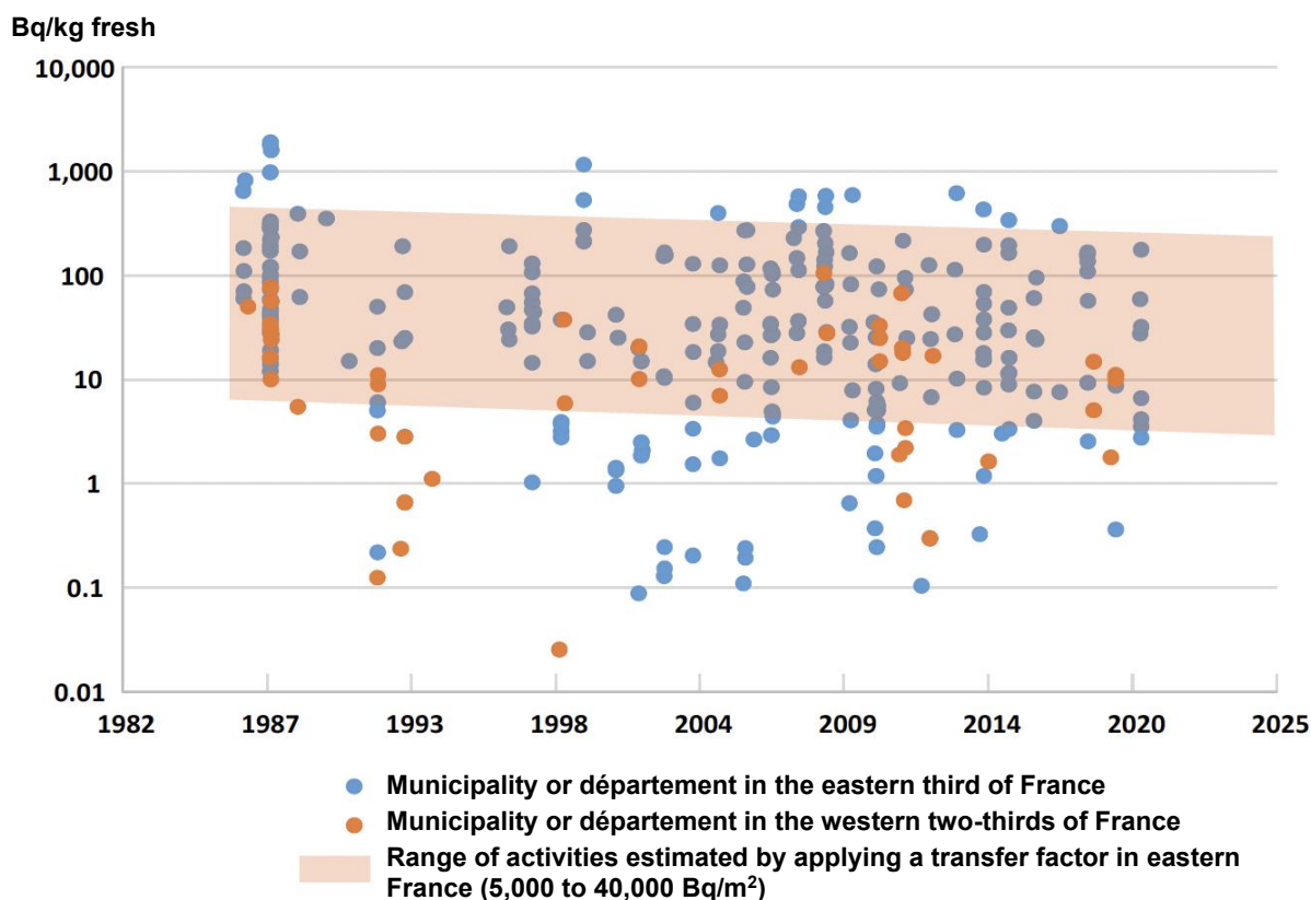
Figure 29: Specific activities of caesium-137 (Bq/kg fresh) measured since 1986 by ASNR (and its predecessors IPSN, OPRI and IRSN) in mushrooms collected in mainland France.
