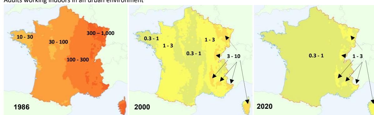
Figure 27: Estimated average effective doses for adults working outdoors in a rural environment (top maps) or indoors in an urban environment (bottom maps) in 1986, 2000, and 2020 (in µSv/year)
