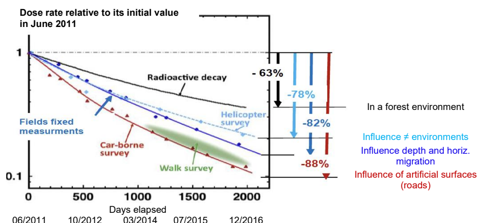
Figure 9: Decrease in dose rate observed in different types of environment by different types of measurement over the five years following the Fukushima accident (from Siato K. et al, 2019)
