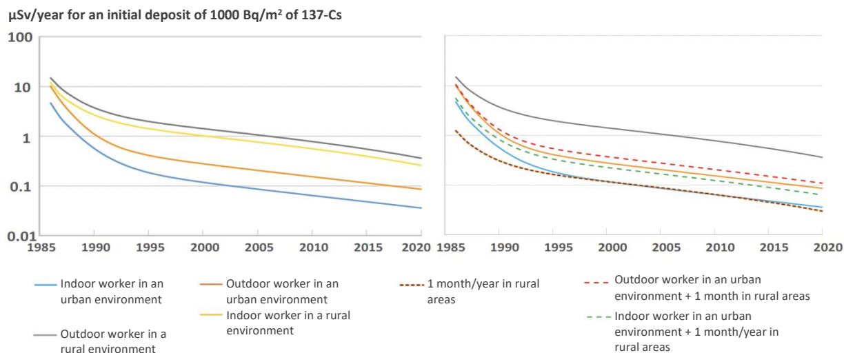
Figure 14: Comparison of average external effective doses ( \mu\text{Sv}/\text{year} ) estimated for adults working outdoors or indoors in rural or urban environments (left graph); taking into account the exposure time (stay) spent by a city dweller on natural surfaces (right graph).
