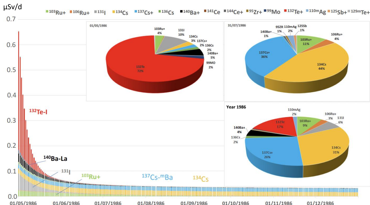
Figure 11: Trend in daily external dose (μSv/d) for an adult working outdoors in a rural environment in 1986 and for a unit deposit of 1 kBq/m² of 137-Cs, with contributions from the various radionuclides
