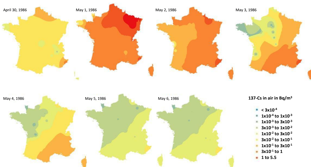
Figure 4: Maps of daily airborne 137 -Cs activity from April 30th to May 6th (Bq/m 3 )
