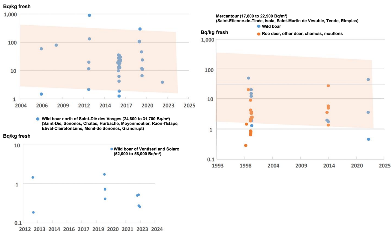
Figure 32: Caesium-137 specific activities (Bq/kg fresh) measured by ASNR (and its predecessors IPSN, OPRI and IRSN) in game meat collected in a number of municipalities or groups of municipalities in eastern France.
